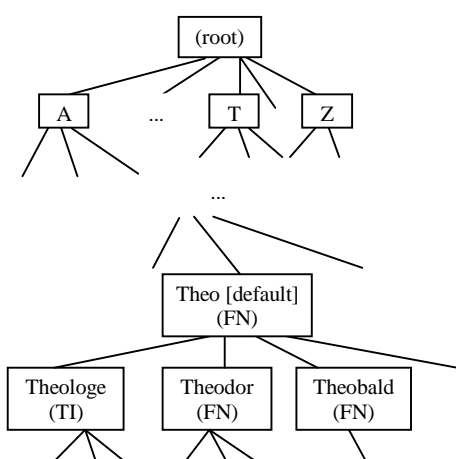
Figure 2: Prefix Decision Tree for Proper Names
